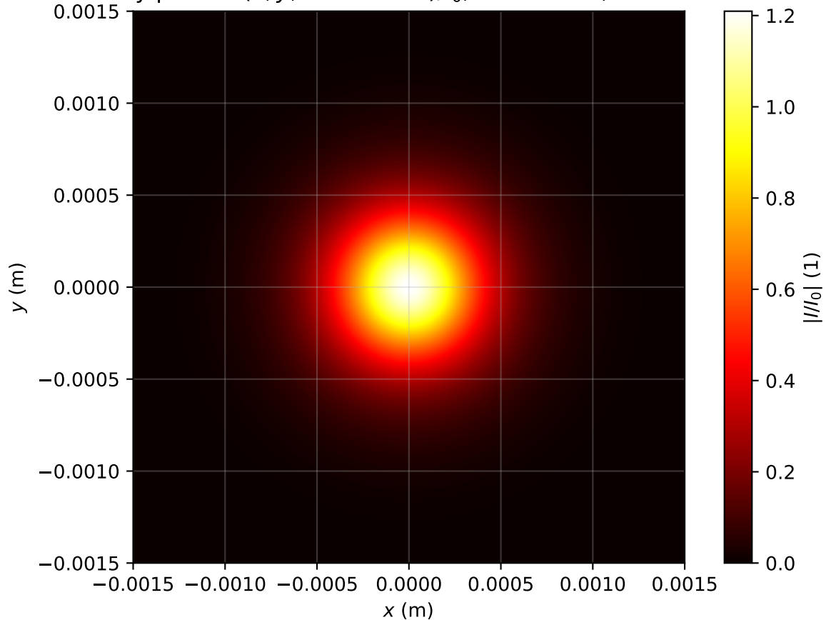
Intensity profile I(x, y, z = 1.115m)/I_0 , Pin=0.7Pcr, artificial time
